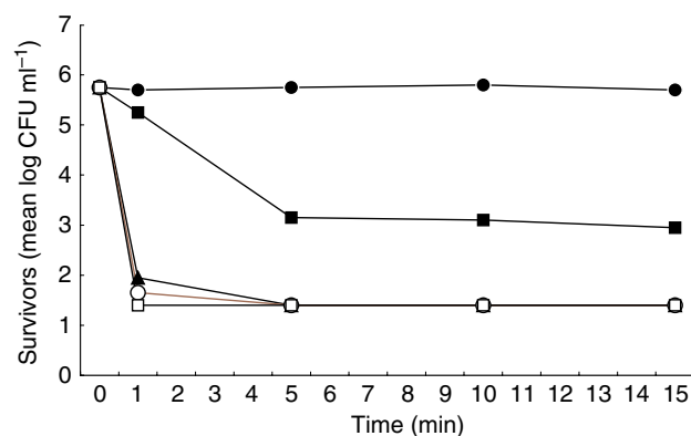
Fig. 1 Survivor curves for E. coli O157:H7 in Mueller-Hinton broth at different concentrations of oregano oil at 37°C: (●) 0 \mu\text{l l}^{-1} (control), (■) 78 \mu\text{l l}^{-1} , (▲) 156 \mu\text{l l}^{-1} , (○) 312 \mu\text{l l}^{-1} , (□) 625 \mu\text{l l}^{-1} oregano oil. The detection limit for viable cells was 1.4 log CFU \text{ml}^{-1} . Where no viable cells were recovered, the detection limit is indicated
