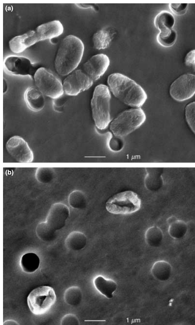
Fig. 2 Scanning electron microscope images of E. coli O157:H7 cells after treatment with oregano essential oil (12 000 ×). (a) Untreated cells (control). (b) Cells damaged after treatment with 625 \mu\text{l l}^{-1} oregano oil
